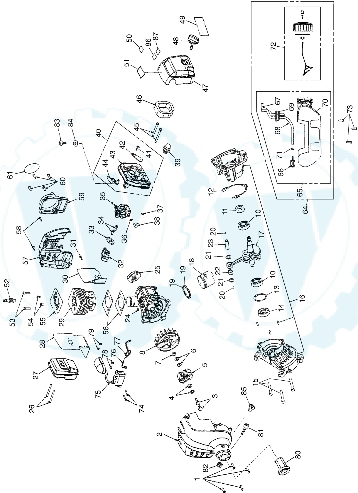
Fig.2 ENGINE GROUP
