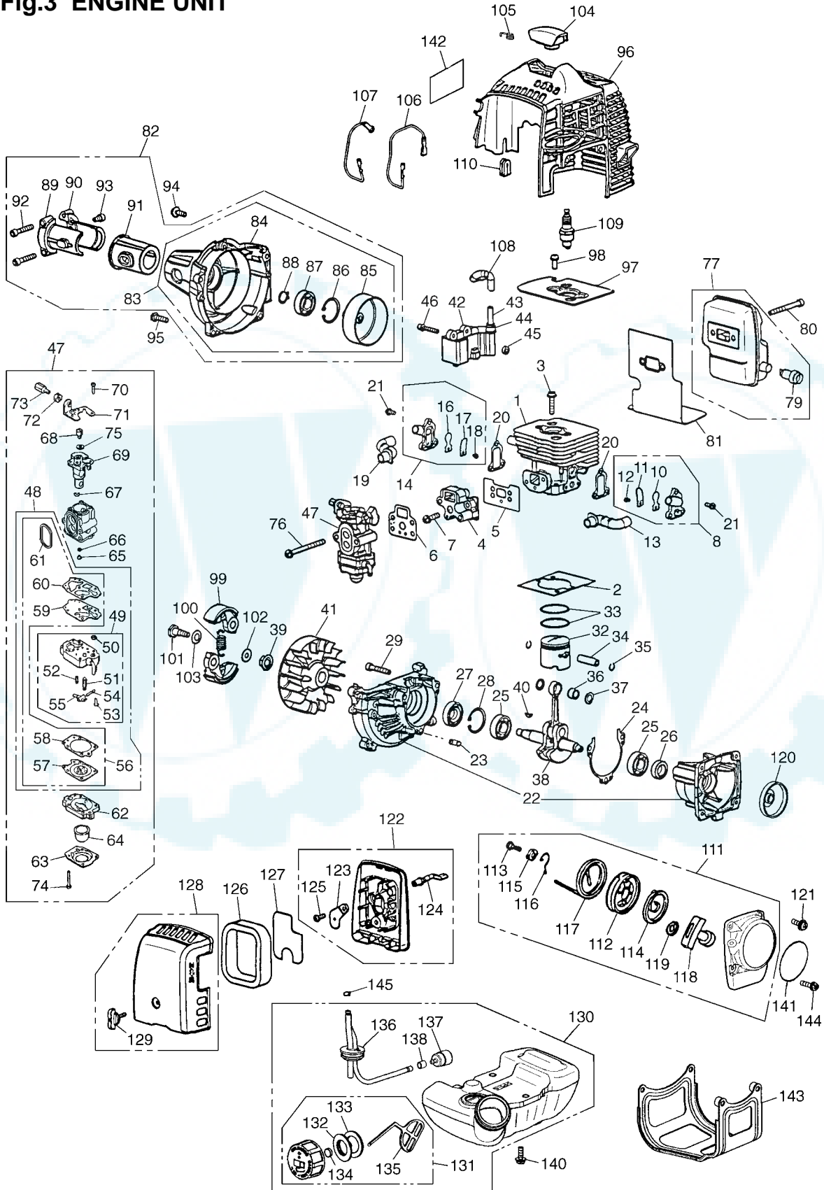
Fig.3 ENGINE UNIT
