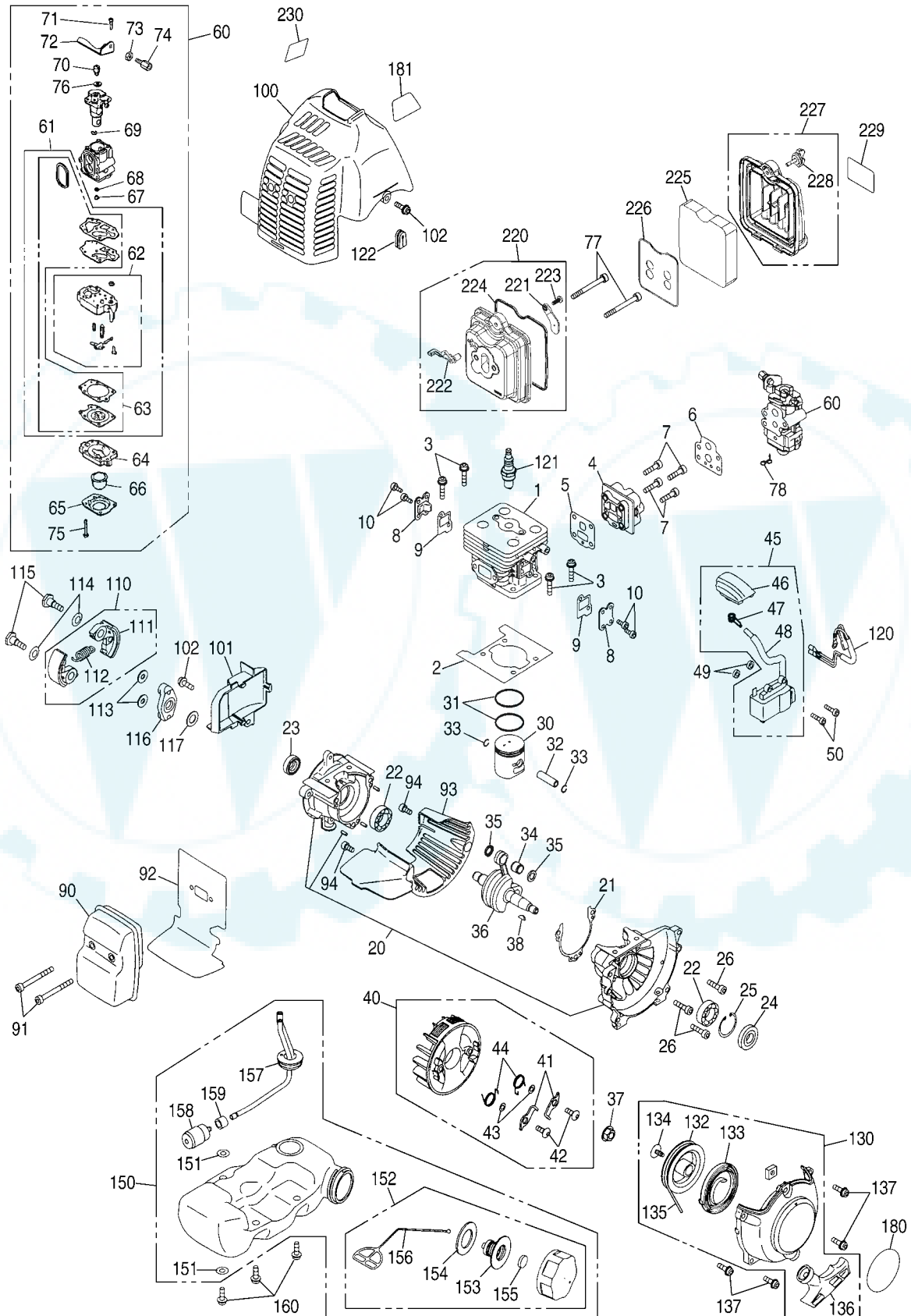
Fig.3 ENGINE UNIT
