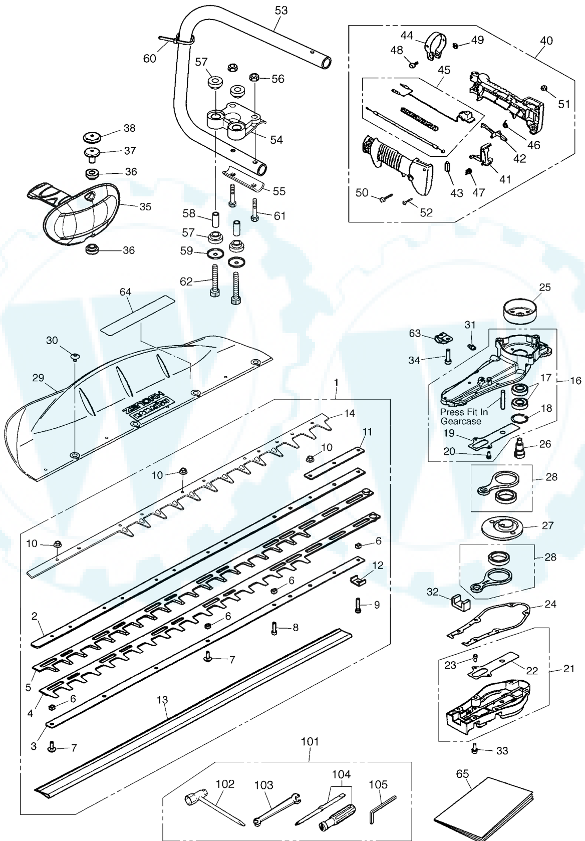
Fig.1 CUTTING UNIT
