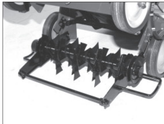
2) Lose Messer.
