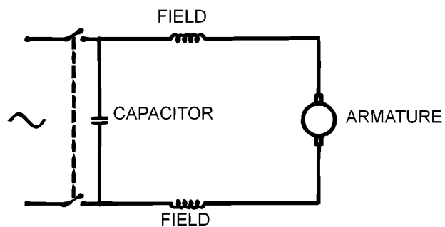
CIRCUIT DIAGRAM
