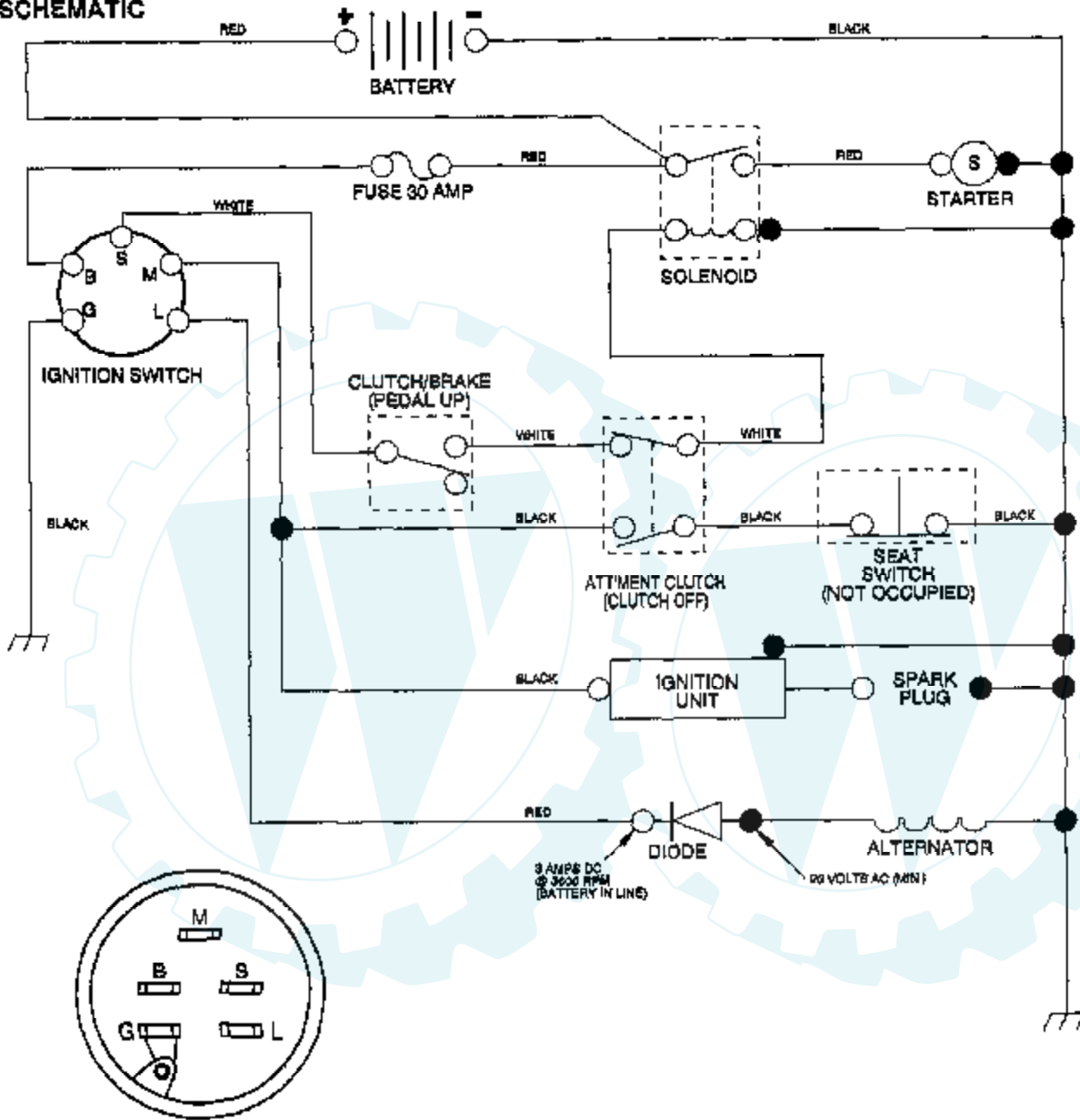
IGNITION SWITCH
