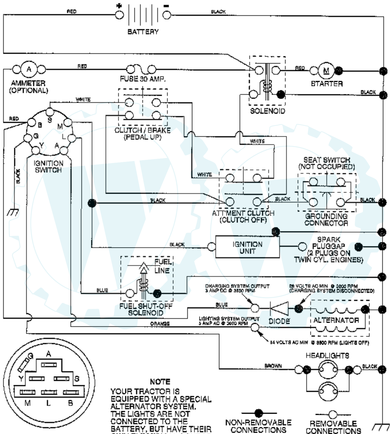
IGNITION SWITCH
