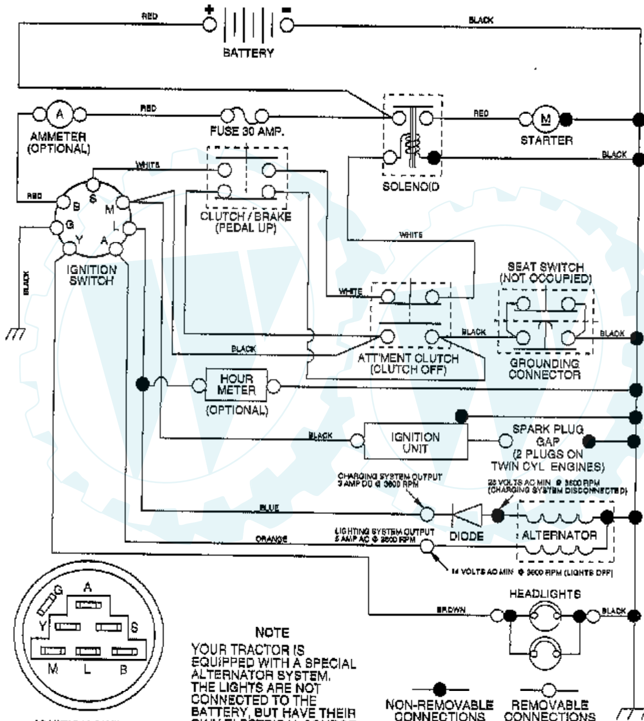
IGNITION SWITCH
