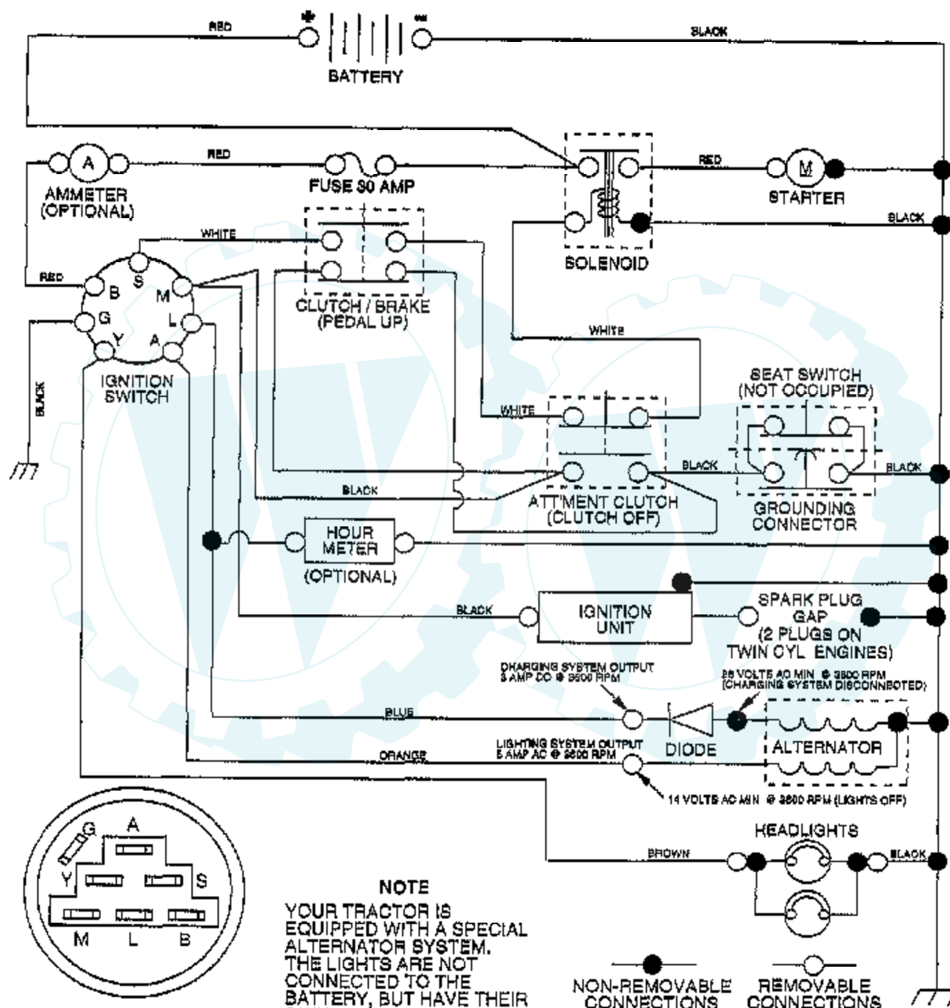
IGNITION SWITCH
