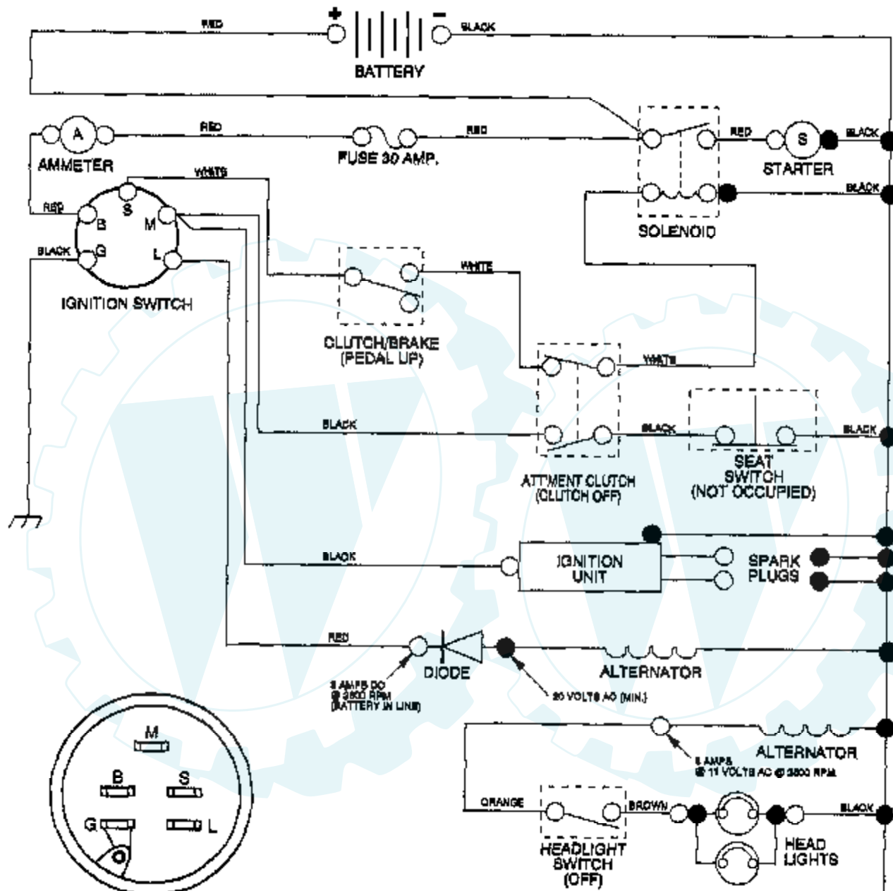
IGNITION SWITCH
