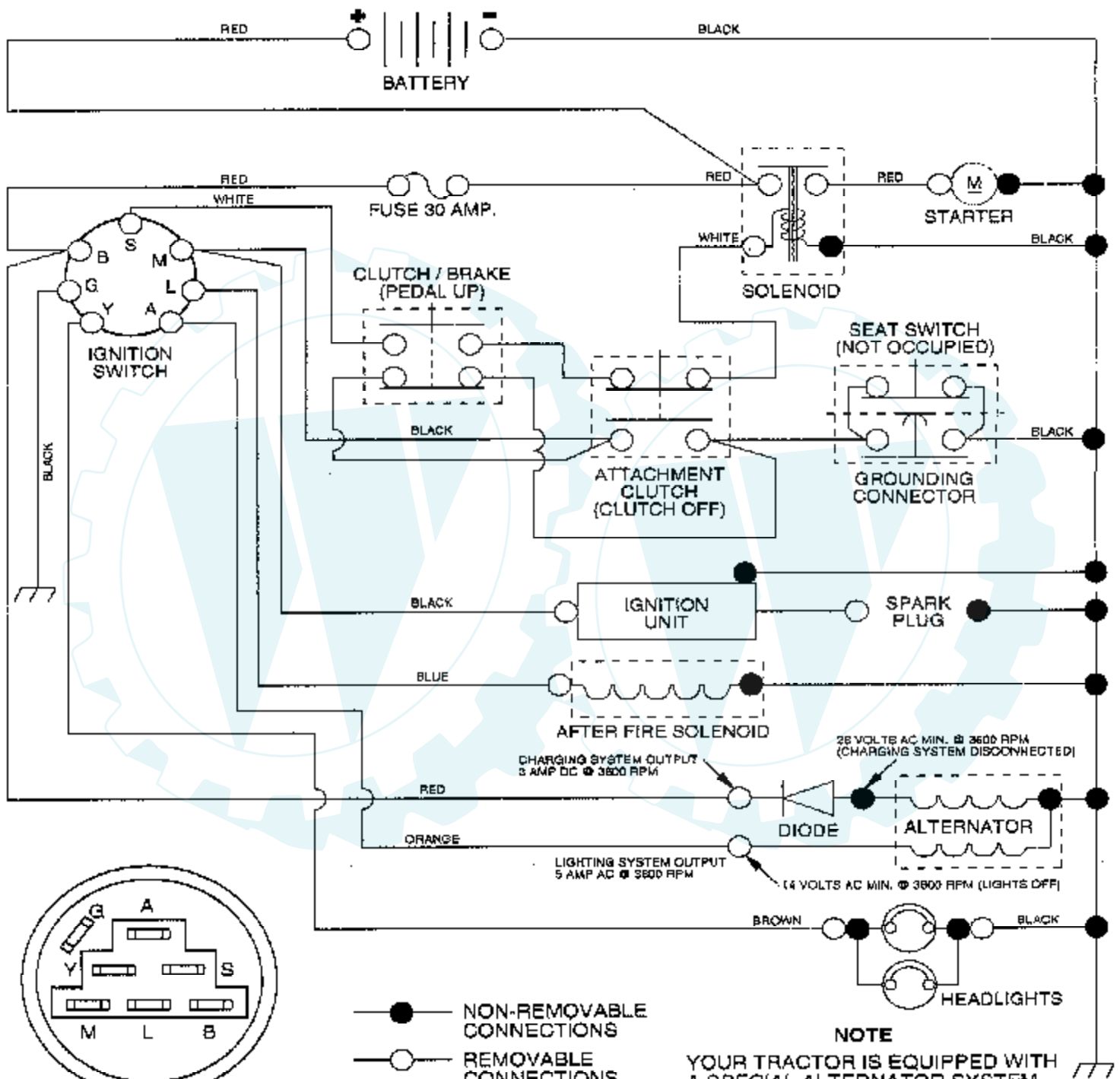
IGNITION SWITCH
