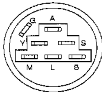
IGNITION SWITCH
