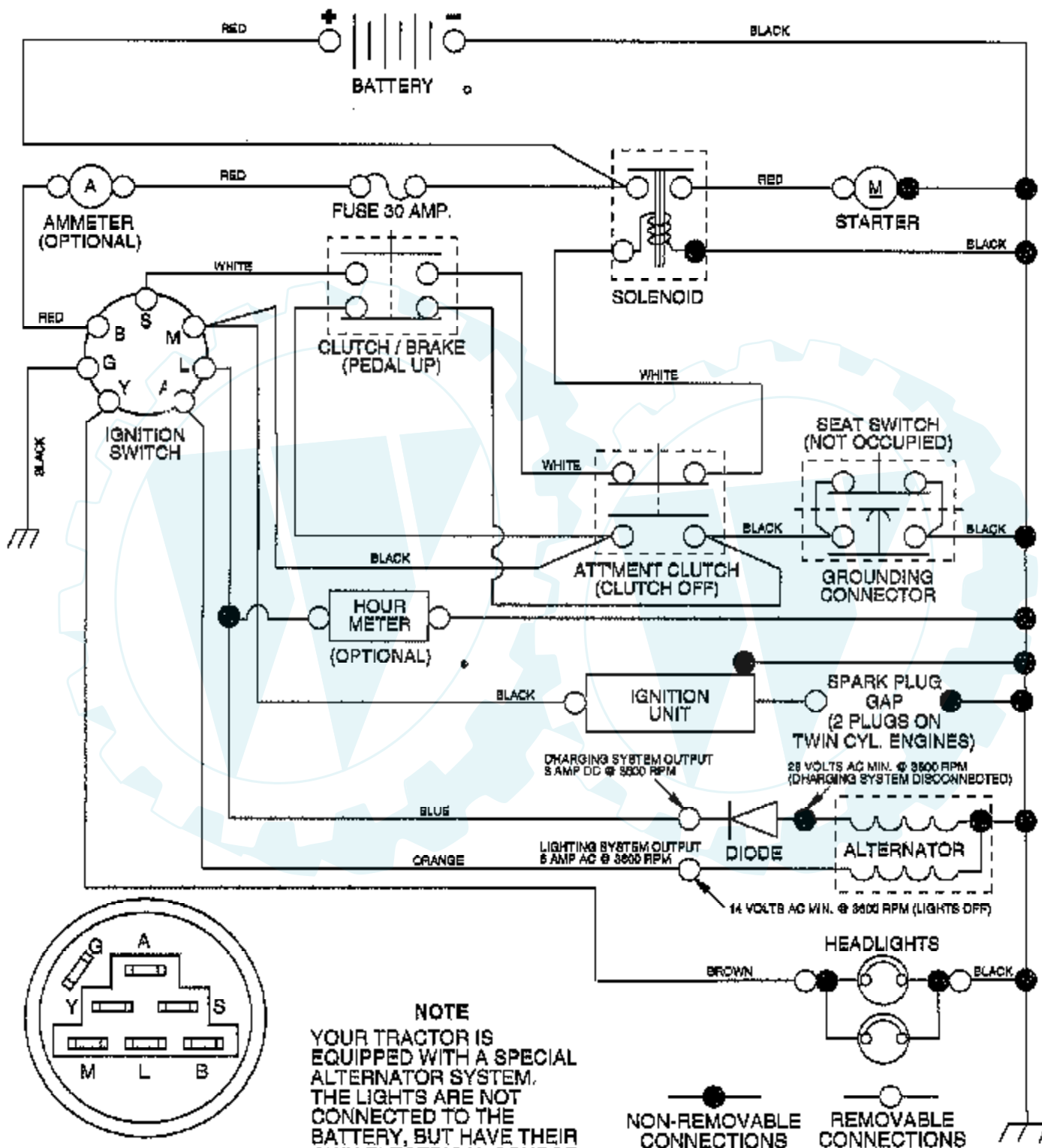
IGNITION SWITCH
