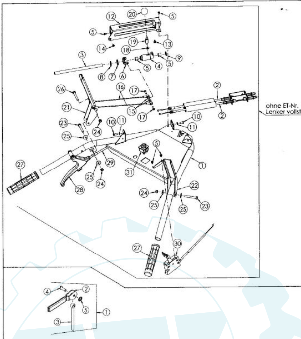
Vormontagegruppen AS 73 vs 05/2001
