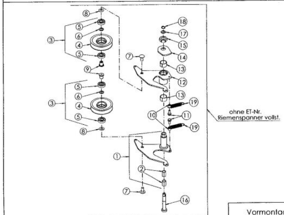
Vormontagegruppen AS 73 vs
